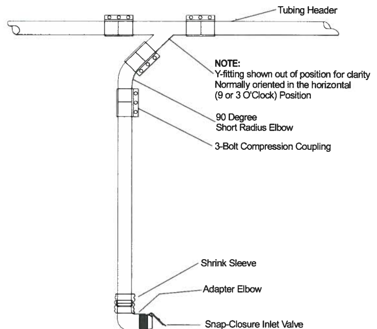
Typical Vacuum Drop with Snap Closure Inlet
